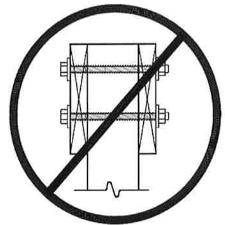
PROHIBITED CONNECTION
