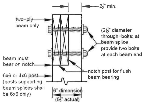
NOTCHED POST
