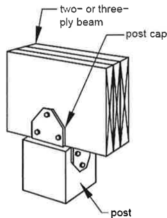
POST CAP
